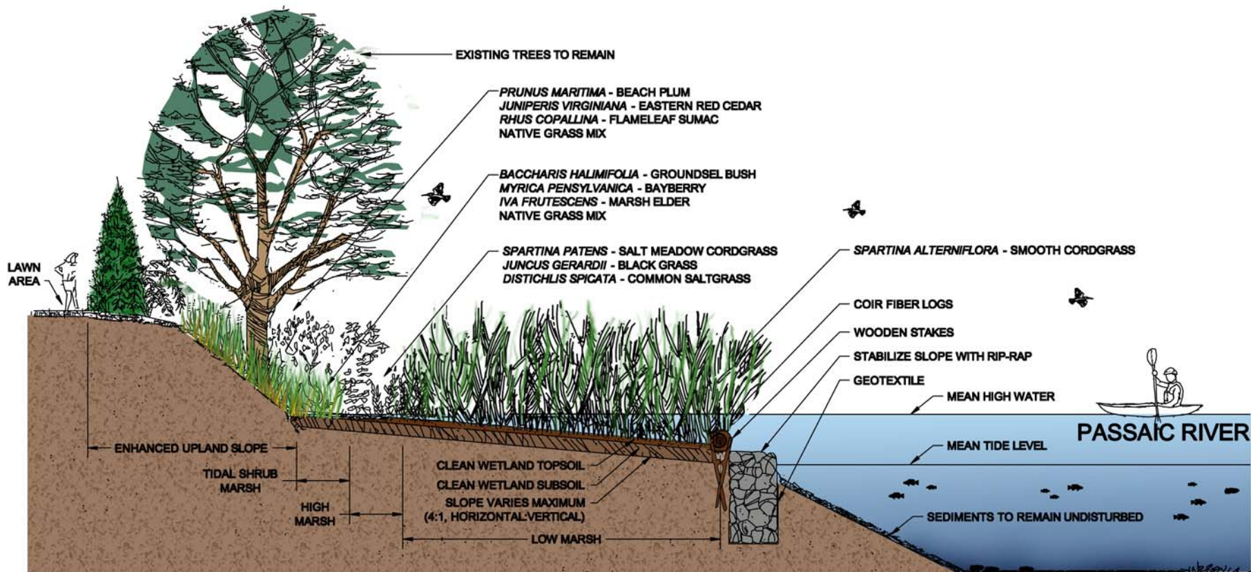
MINISH (AFTER RESTORATION) NOT TO SCALE
