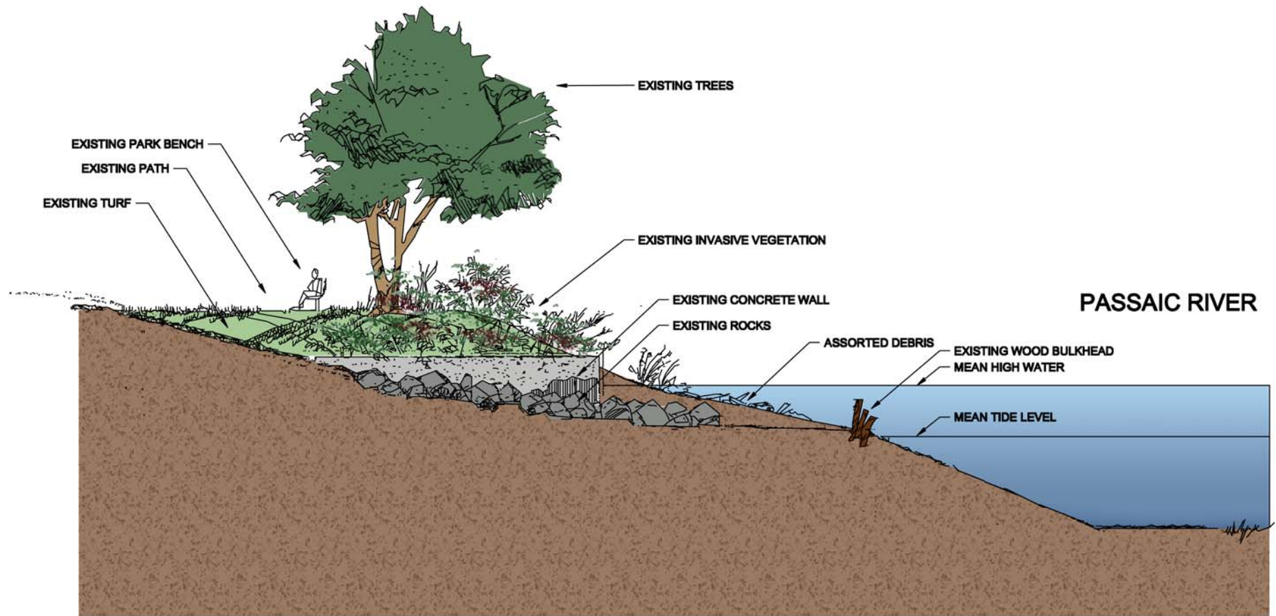
KEARNY BOAT RAMP (BEFORE RESTORATION) NOT TO SCALE
